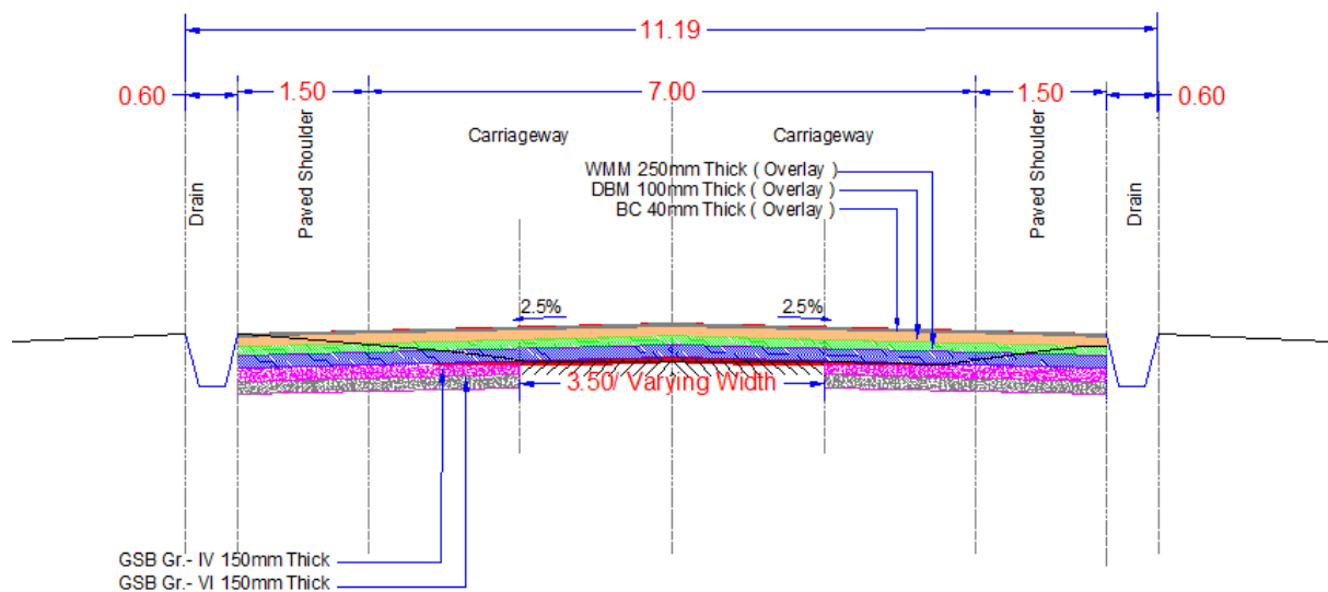
Figure 36: TYPICAL CROSS-SECTION 2A
