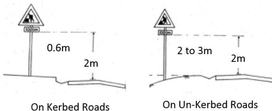
Figure DEVICES USED IN CONSTRUCTION ZONES
