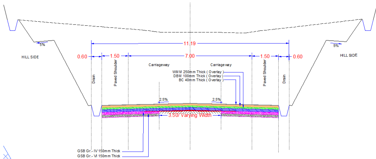
Figure 6: Typical Cross-section 3
