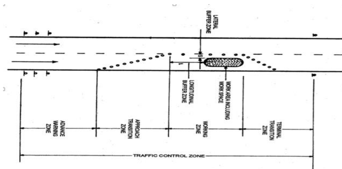
Figure 44: ELEMENT OF TRAFFIC CONTROL ZONE
