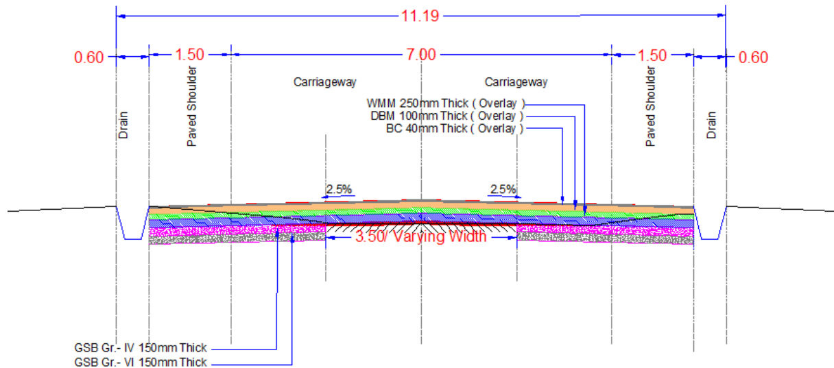
Figure 5: Typical Cross-section 2B
