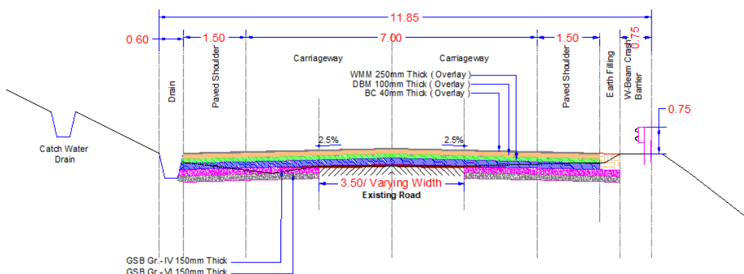
Figure 3: TYPICAL CROSS-SECTION 2
