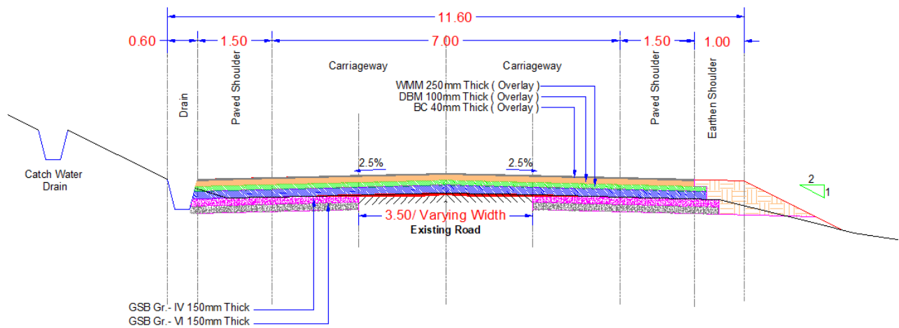
Figure 38: Typical Cross-section 3B
