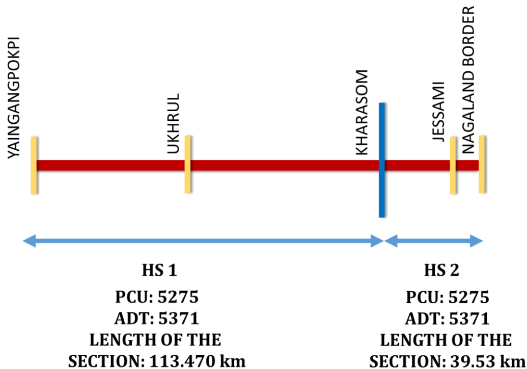
Figure 33: PROJECT ROAD WITH HOMOGENEOUS SECTIONS
