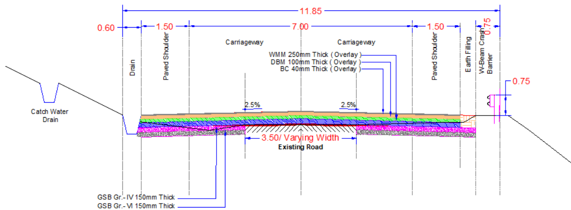
Figure 34: TYPICAL CROSS SECTION 1
