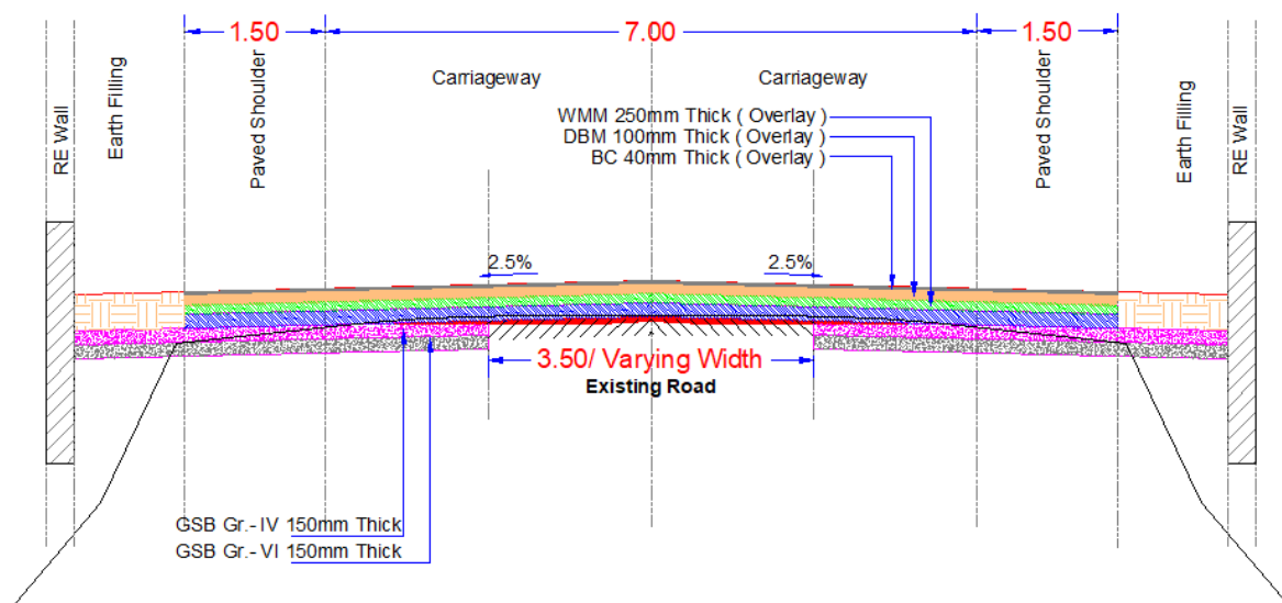
Figure 14: Typical Cross-section 8
