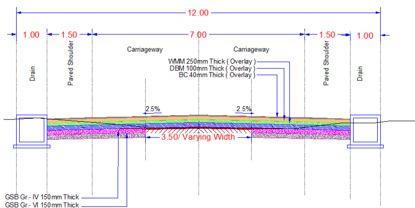
Figure 4: TYPICAL CROSS-SECTION 2A
