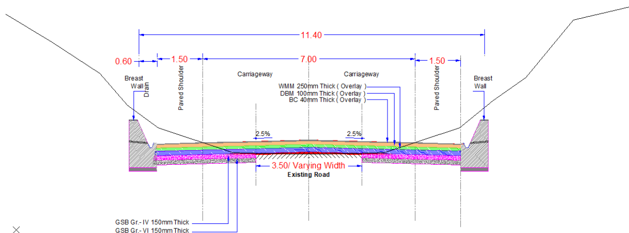
Figure 43: Typical Cross-section 8
