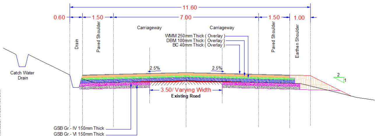
Figure 6: Typical Cross-section 3
