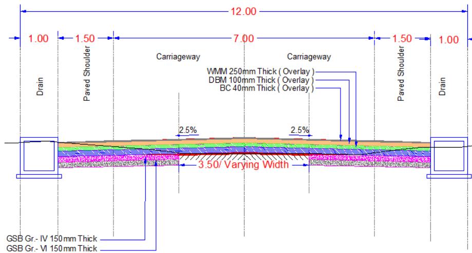
Figure 36: TYPICAL CROSS-SECTION 2A
