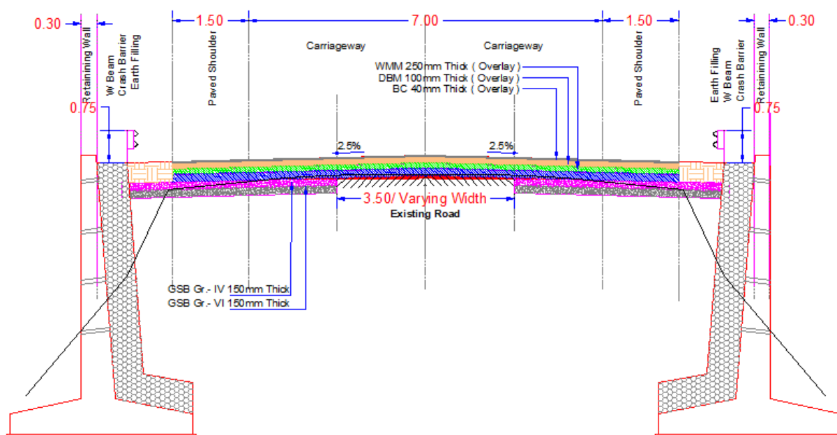
Figure 12: Typical Cross-section 7
