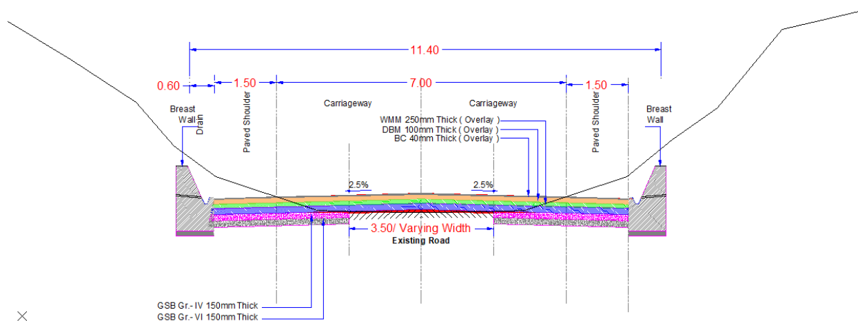
Figure 14: Typical Cross-section 8
