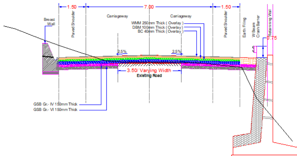
Figure 39: Typical Cross-section 4
