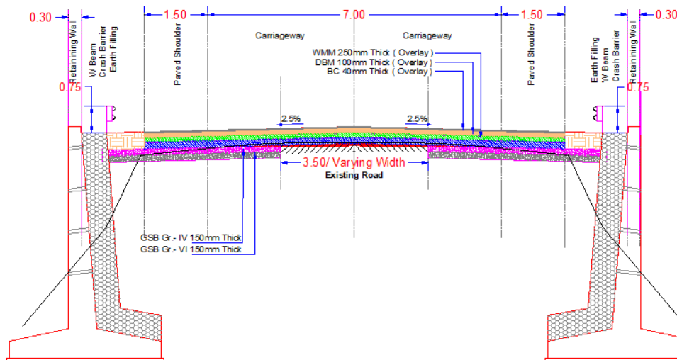
Figure 42: Typical Cross-section 7A
