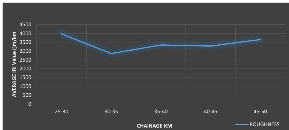
Figure 23: ROUGHNESS VALUE
