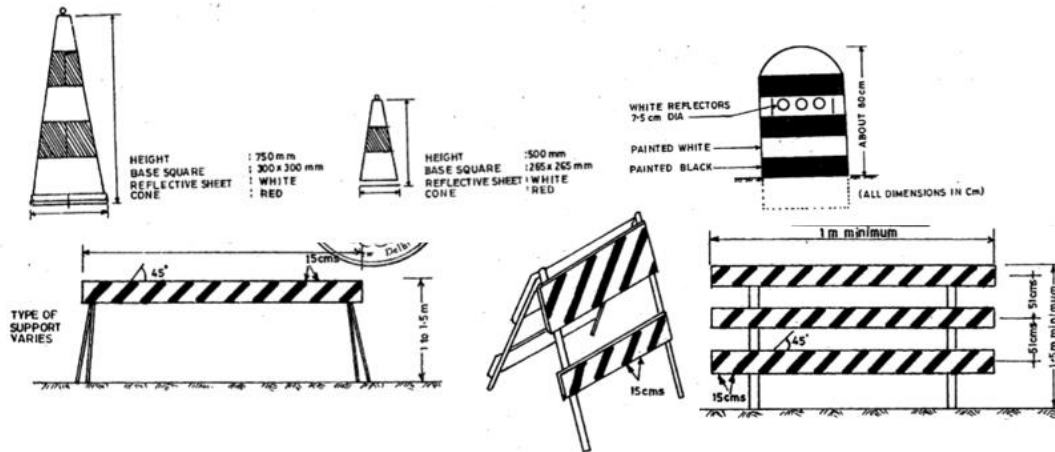
Figure 48: FLAGMEN AT CONSTRUCTION ZONE
