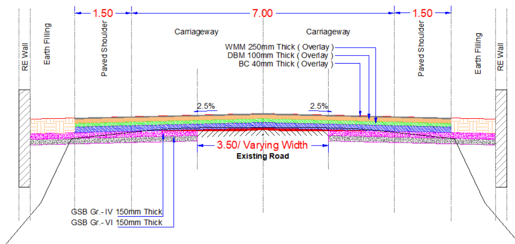
Figure 42: Typical Cross-section 7A
