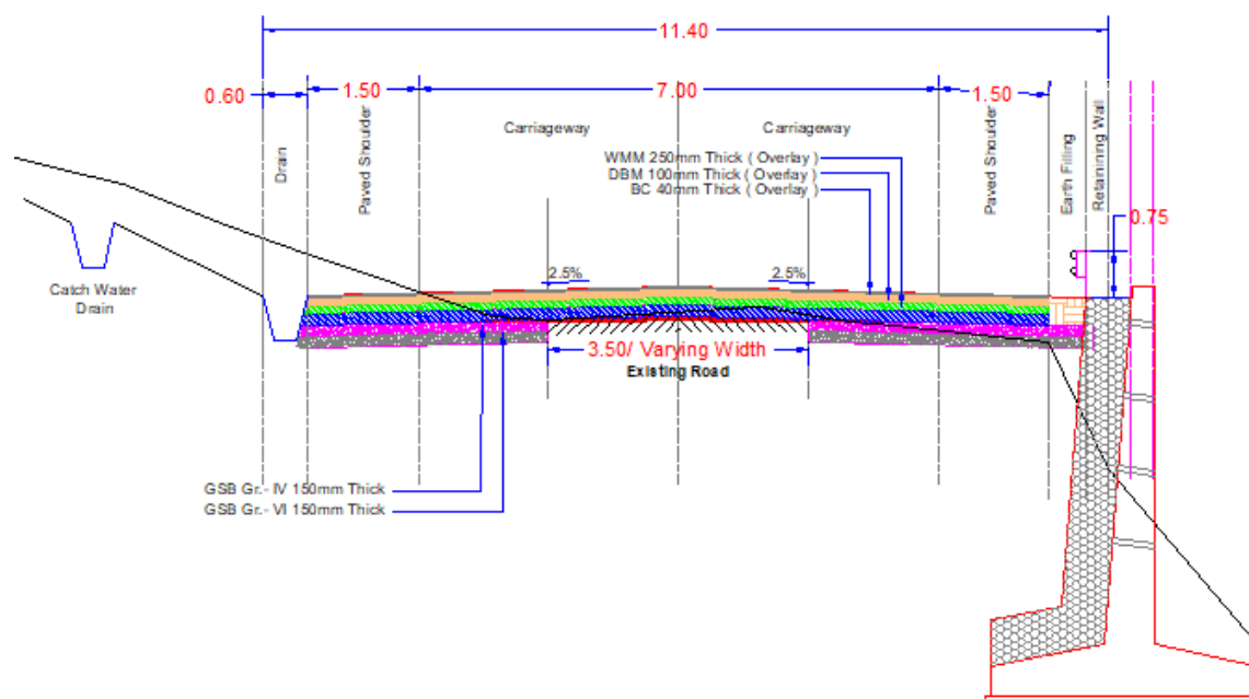
Figure 10: Typical Cross-section 5
