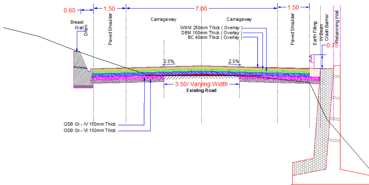
Figure 12: Typical Cross-section 7
