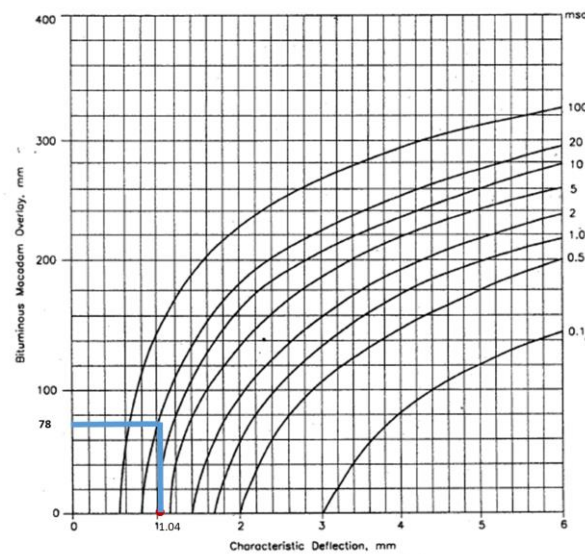
Figure 24: OVERLAY CALCULATION
