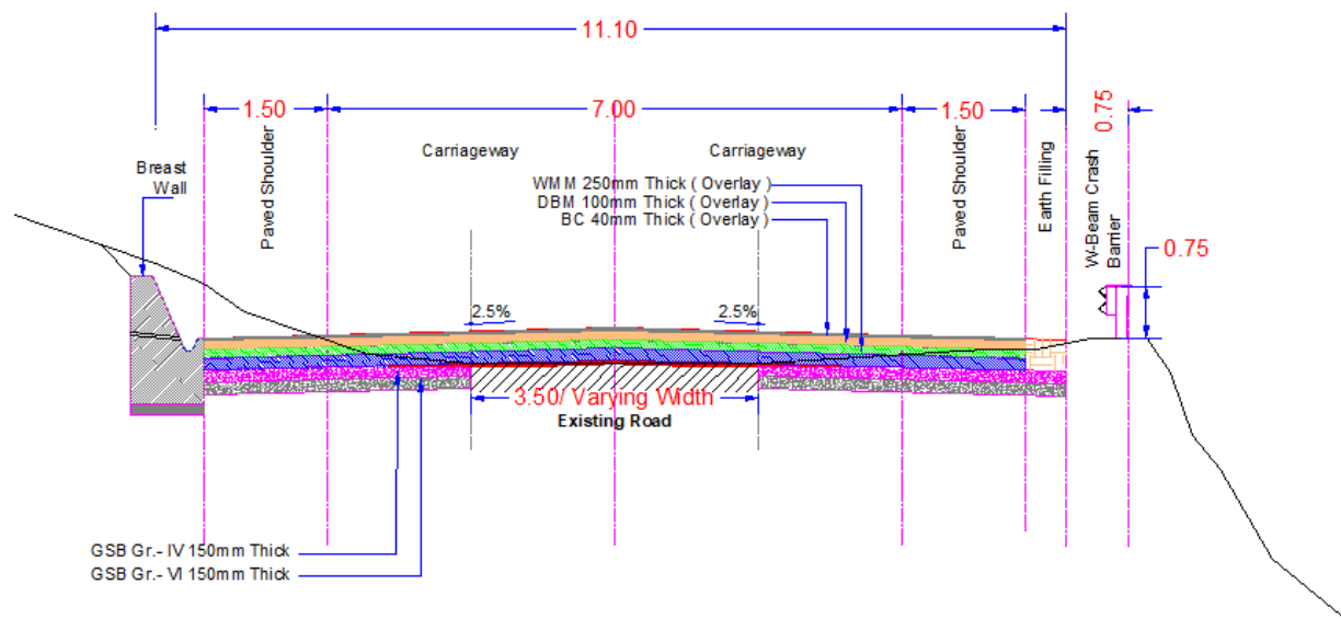
Figure 10: Typical Cross-section 5
