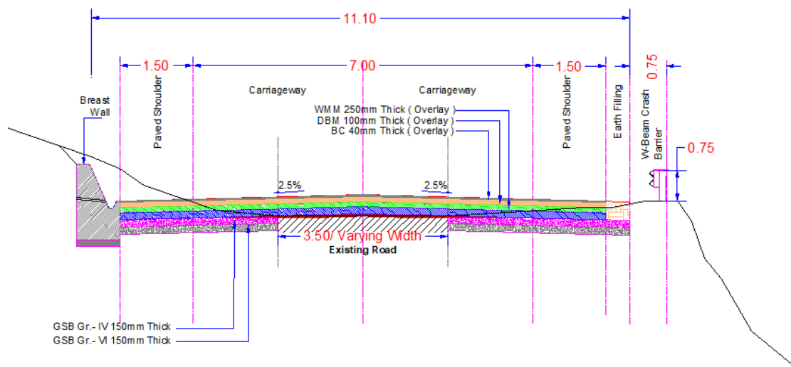
Figure 39: Typical Cross-section 4
