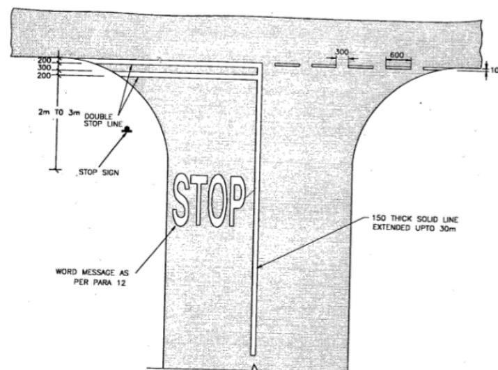
Figure 51: ROAD MARKINGS FOR STOP SIGNS
