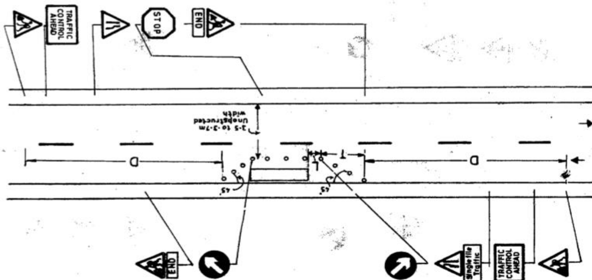
Figure 49: TRAFFIC CONTROL BY STOP/GO BOARDS
