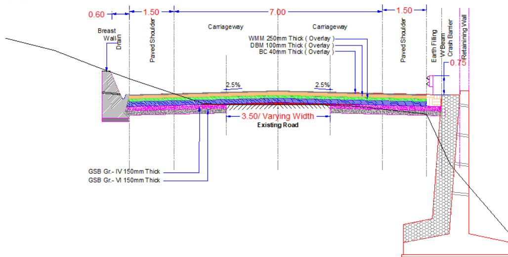
Figure 41: Typical Cross-section 7
